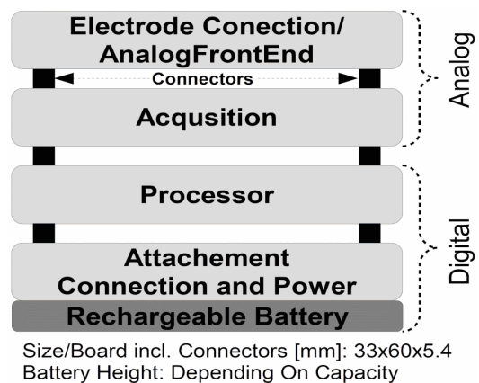
Figure 3: Module stack of the embedded data acquisition and identification module
