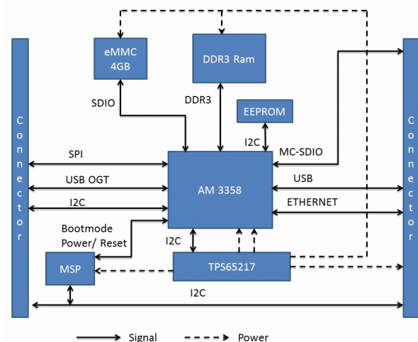
Figure 4: CPU-Module: Processor Board
