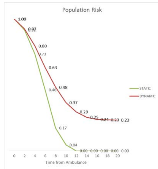
Figure 3: Software output: Static vs Dynamic Population Risk
