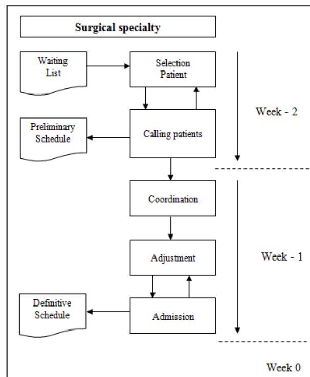
Fig.1: Flowchart process scheduling
